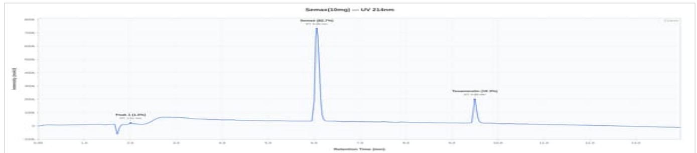
Semax 10mg - LOT-2026-02: UV Chromatogram
